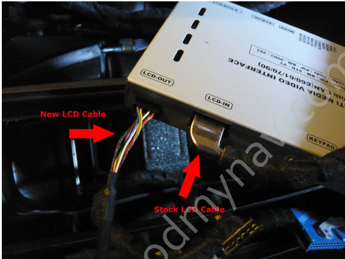
18. Connect LCD Cables to interface module (New LCD Cable to LCD-OUT and Stock LCD Cable to LCD-IN)
