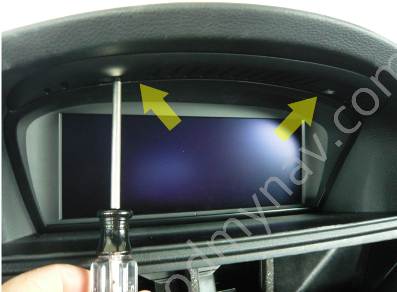
4. Unscrew two screws (Trox #10)
