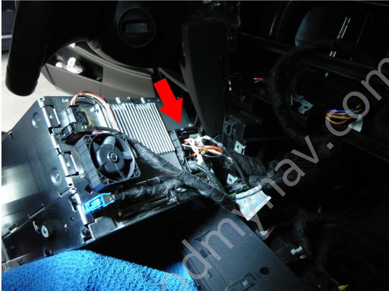
10. Remove stock audio harness
