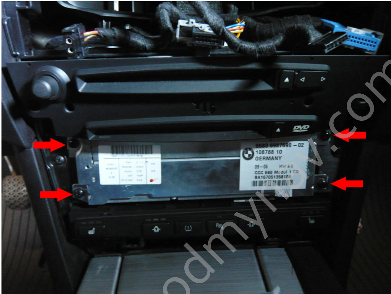
9. Unscrew 4 screws and pull the radio unit towards you
