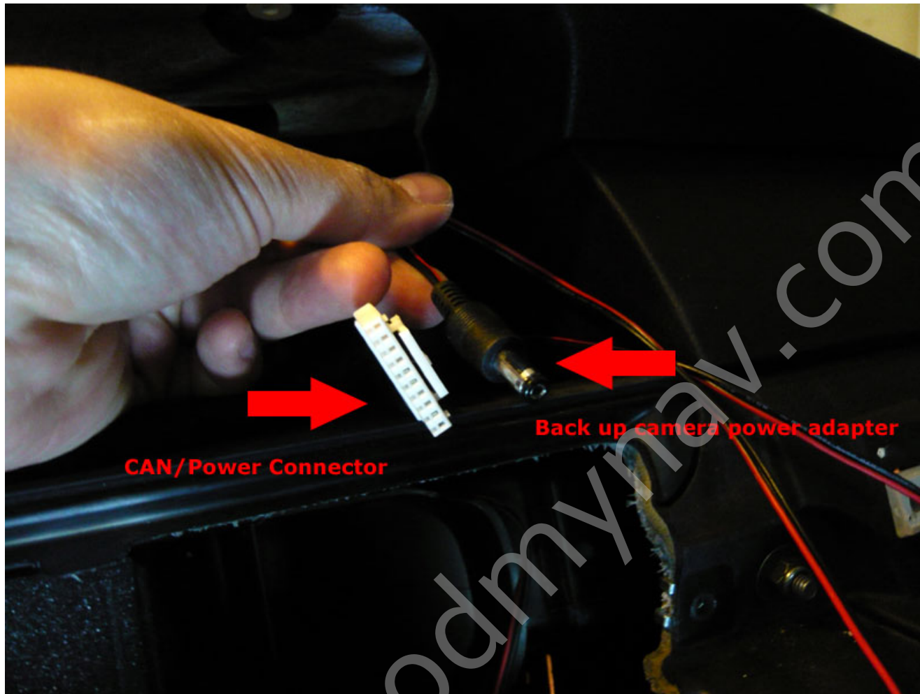
14. Run CAN/Power connector and Back up camera power adapter from radio mount area to your screen area
