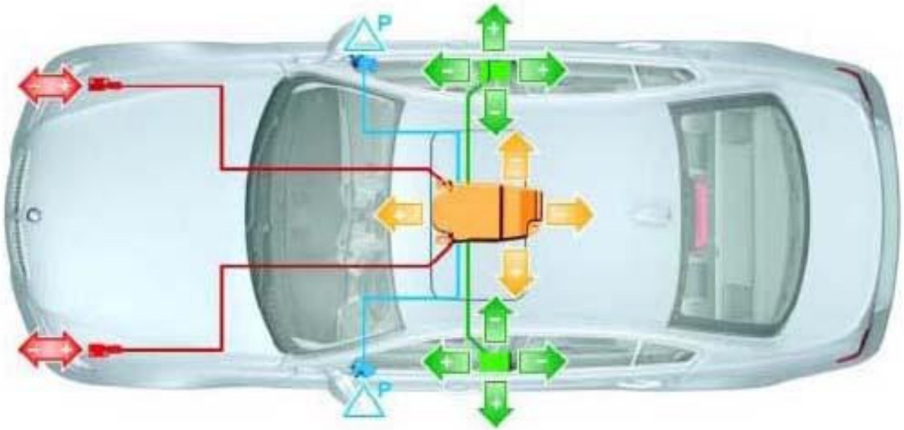
Fig. 27: Identifying Up-Front Sensors Locations Courtesy of BMW OF NORTH AMERICA, INC.
