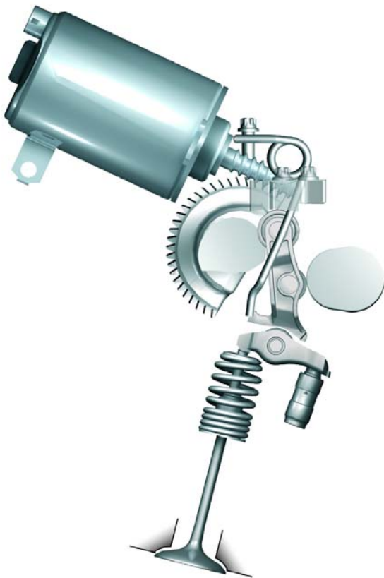
Valvetronic II at minimum valve lift
