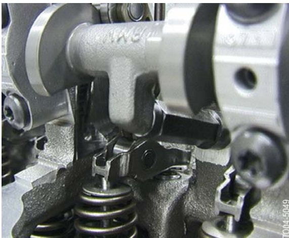
Eccentric Shaft - MIN Stop
