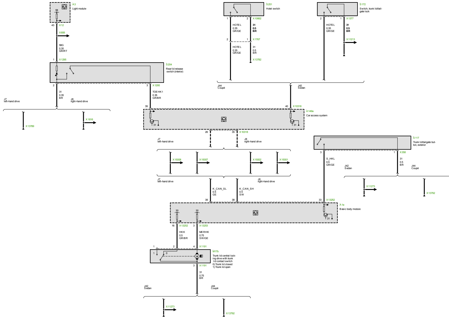
E60 E61 Central locking, trunk lid/tailgate
