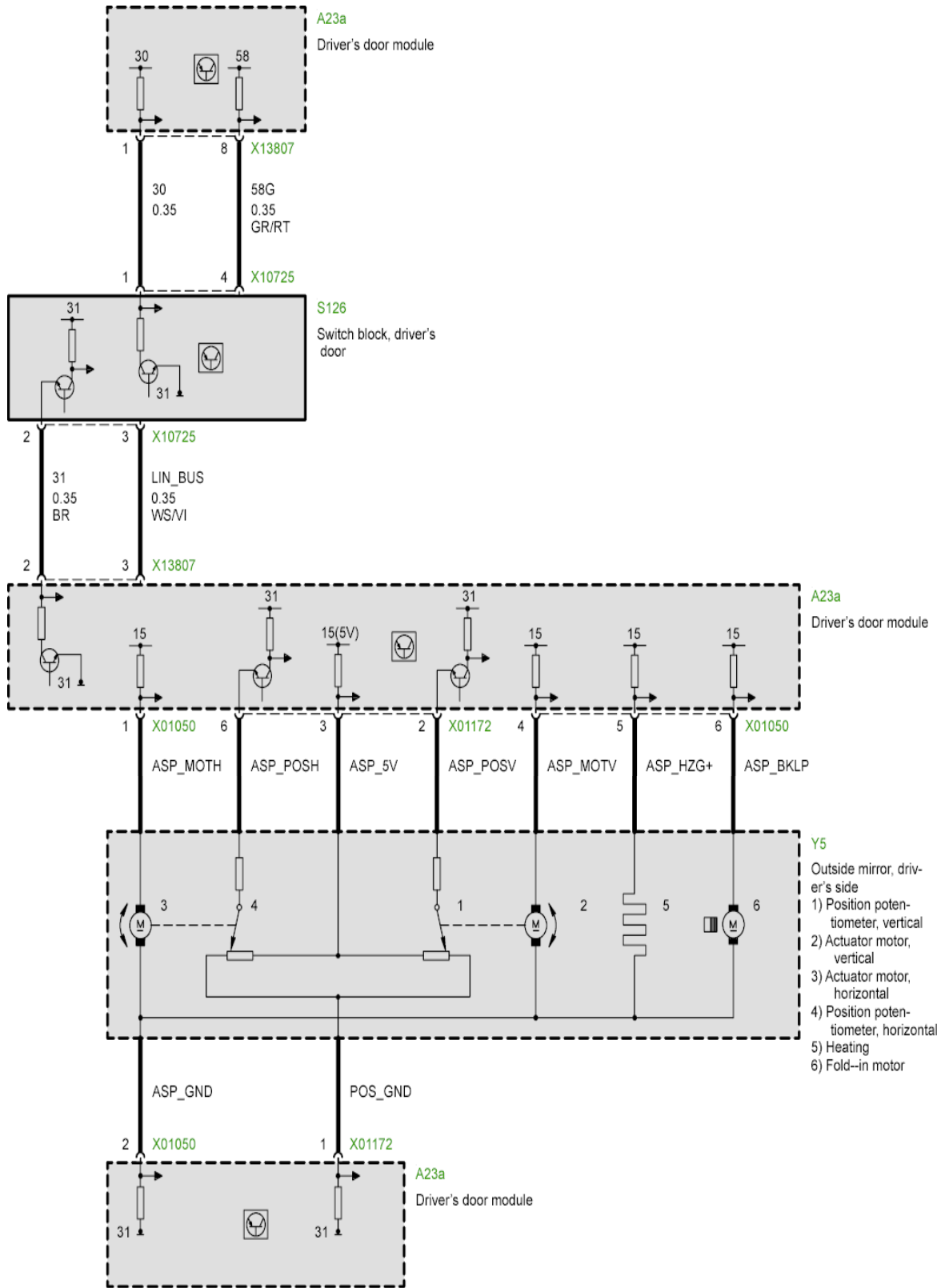
E60 E61 Electric outside mirror, driver's side
