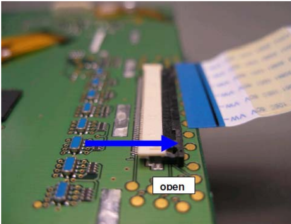
Drive M3.5 (old) connector open
