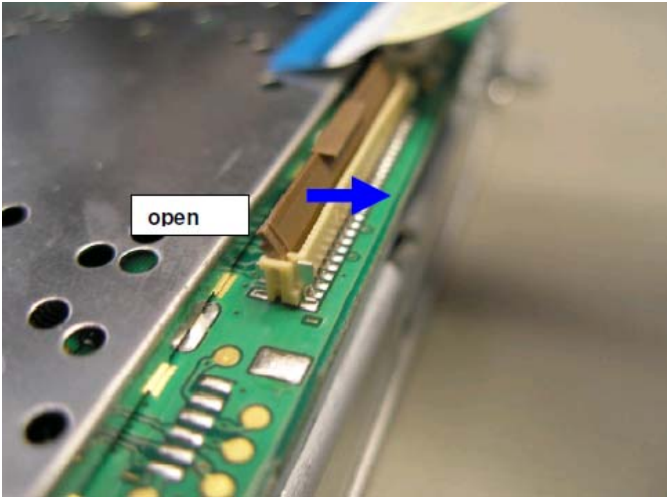
Drive M5 (new) connector open
